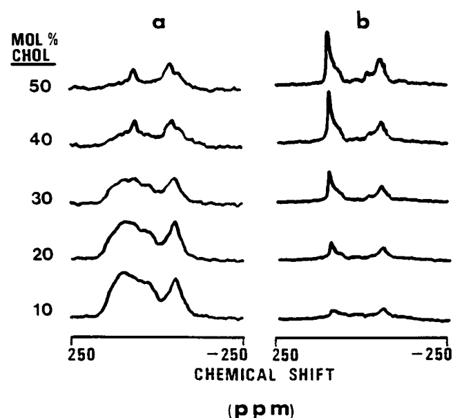
FIGURE 2 Proton decoupled ^{13}\text{C} -NMR spectra of [1-^{13}\text{C}]\text{NPGS/CHOL} mixtures ( T = 70^{\circ}\text{C} ) using (a) cross-polarization with a refocusing pulse or (b) simple Hahn echo pulse sequence.
