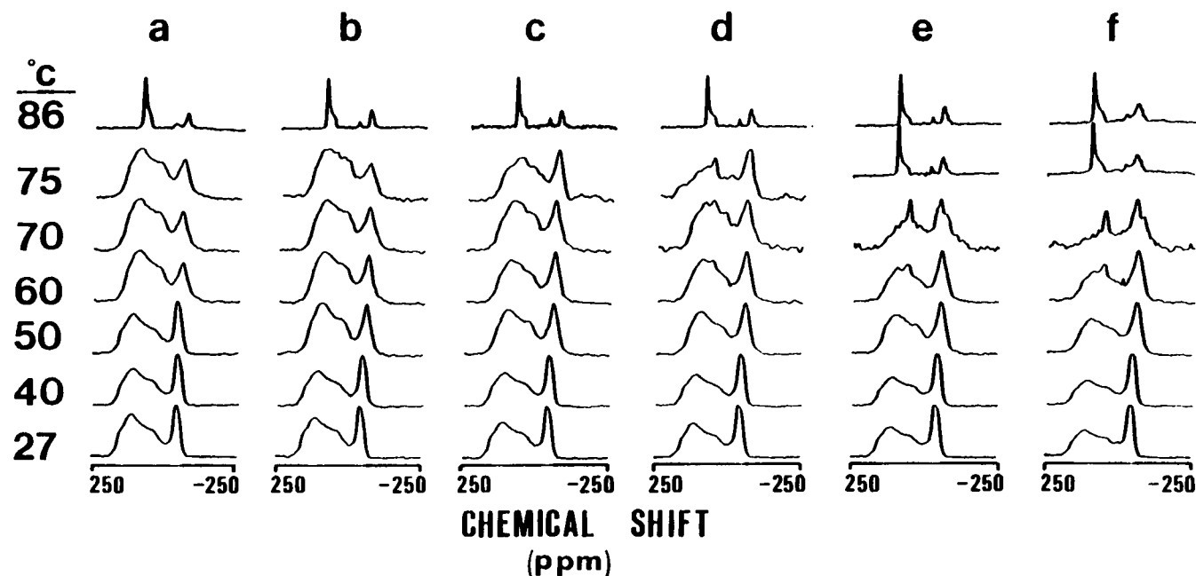
FIGURE 1 Proton-decoupled ^{13}\text{C} -NMR spectra of [1-^{13}\text{C}]\text{NPGS} and [1-^{13}\text{C}]\text{NPGS/CHOL} mixtures as a function of temperature ( ^{\circ}\text{C} ). (a) 0, (b) 10, (c) 20, (d) 30, (e) 40, (f) 50 mol% CHOL.
